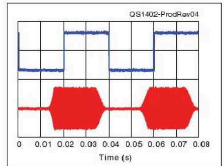
Figure 2 — CW keying waveform for the TS-990S showing the first two dits in full-break-in (QSK) mode using external keying. Equivalent keying speed is 60 WPM. The upper trace is the actual key closure; the lower trace is the RF envelope. (Note that the first key closure starts at the left edge of the figure.) Horizontal divisions are 10 ms. The transceiver was being operated at 200 W output on the 14 MHz band.
