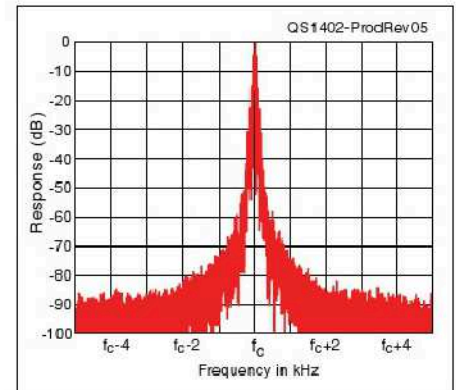
Figure 3 — Spectral display of the TS-990S transmitter during keying sideband testing. Equivalent keying speed is 60 WPM using external keying. Spectrum analyzer resolution bandwidth is 10 Hz, and the sweep time is 30 seconds. The transmitter was being operated at 200 W PEP output on the 14 MHz band, and this plot shows the transmitter output \pm 5 kHz from the carrier. The reference level is 0 dBc, and the vertical scale is in dB.
